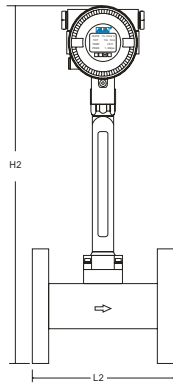
Flange Type
